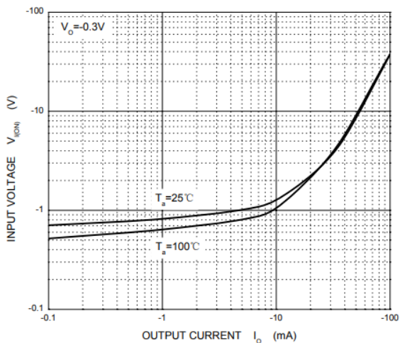
Fig 1: ON Characteristics
