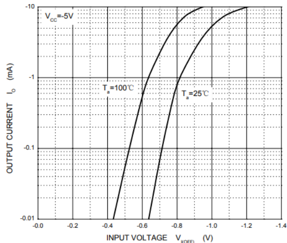
Fig 2: OFF Characteristics
