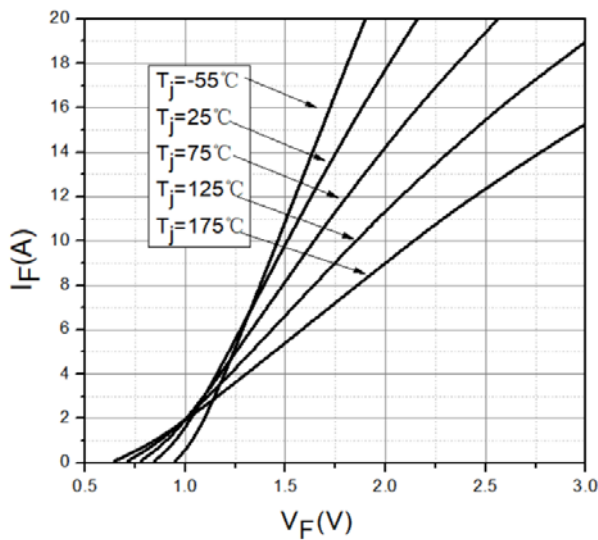
Figure 1. Forward Characteristics
